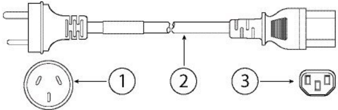
Figure 4: CAB-250V-10A-CH (China)
