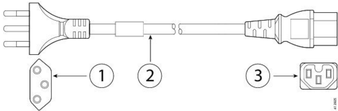
Figure 14: CAB-9K10A-SW (Switzerland)
