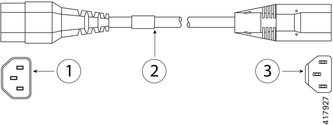
Figure 18: CAB-C13-C14-AC (9.8-foot C13-C14 Cabinet Jumper Power Cord)
