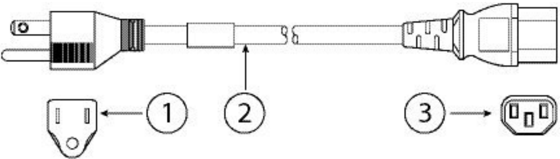
Figure 9: CAB-JPN-3PIN (Japan)
