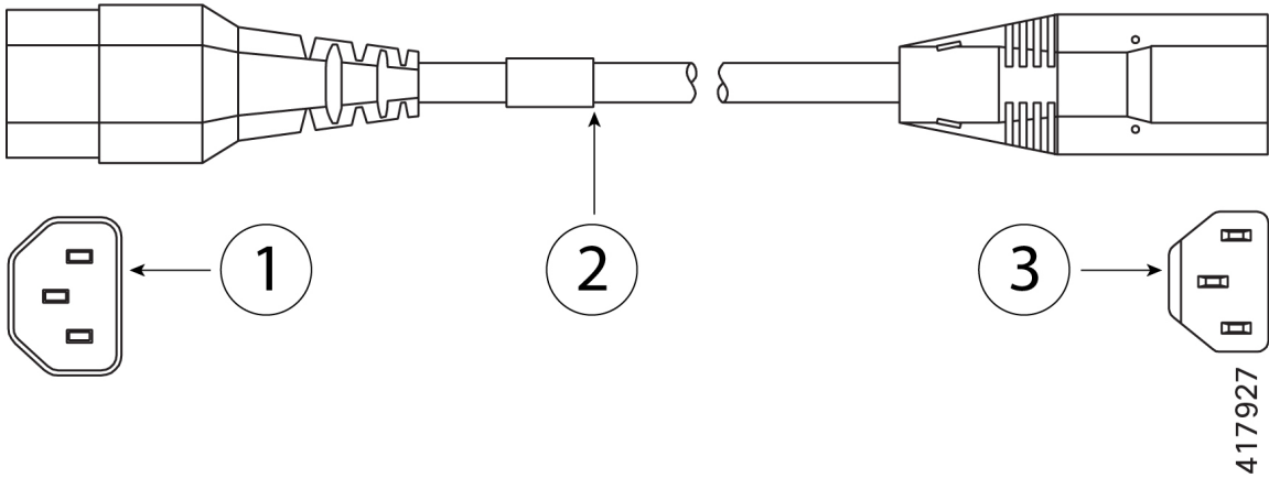
Figure 16: CAB-C13-CBN (2.2-foot C13-C14 Cabinet Jumper Power Cord)
