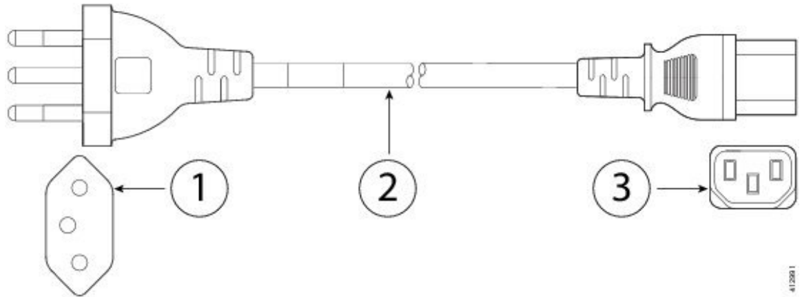
Figure 3: PWR-250V-10A-BZ (Brazil)
