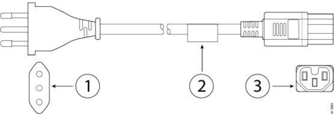
Figure 8: CAB-9K10A-IT (Italy)
