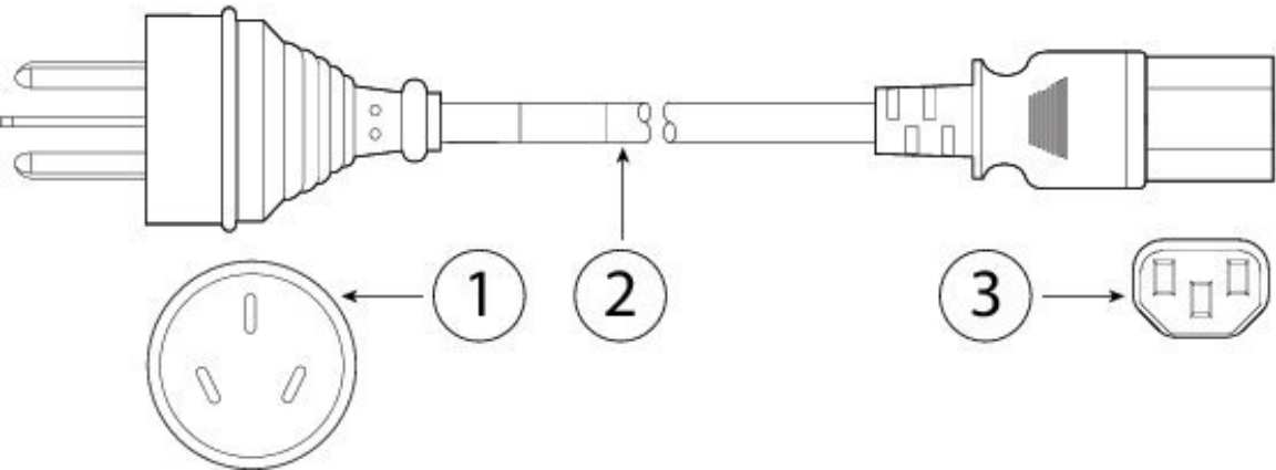
Figure 1: CAB-250V-10A-AR (Argentina)
