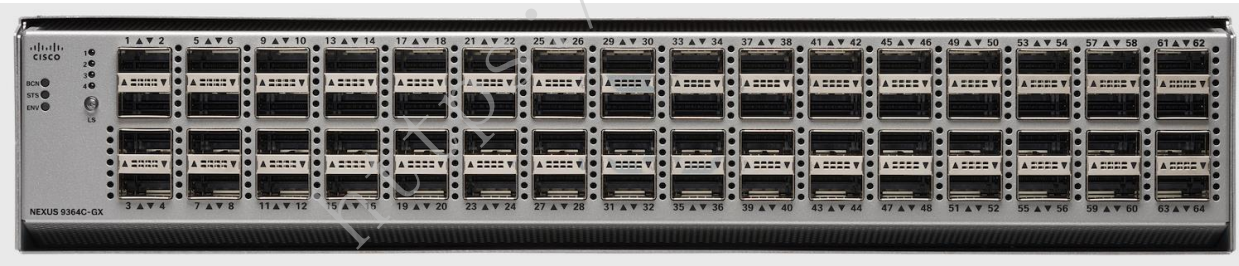
Figure 3. Cisco Nexus 9364C Switch
